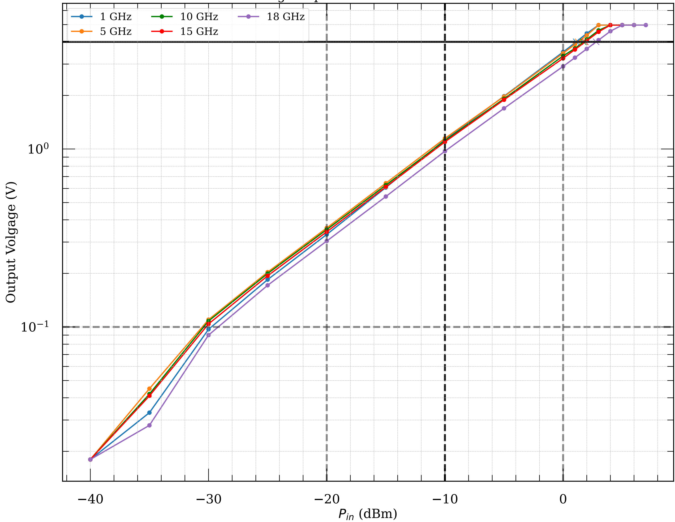
Measured voltage-to-power curve of detector module066v2
